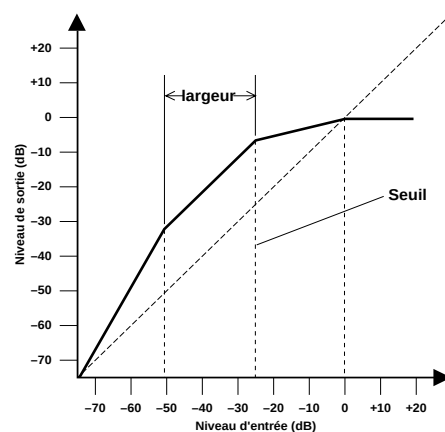
Soft Compander
